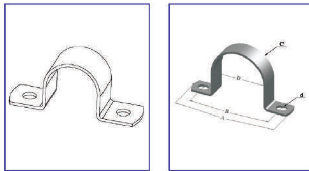
DIMENSIONAL DATA FOR U-STRAP CLAMP (Table No: B-11-01)
